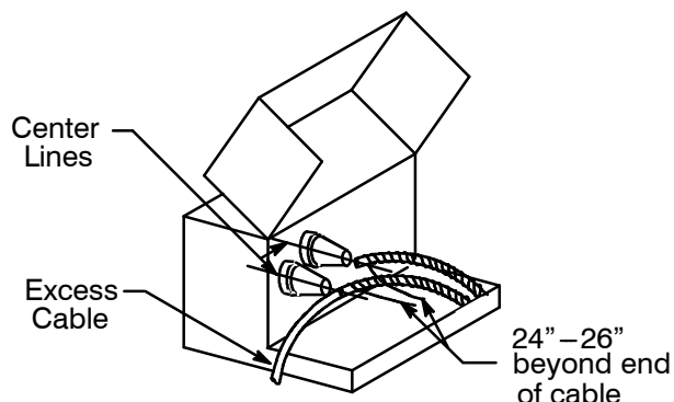
Pad Mount Transformer
