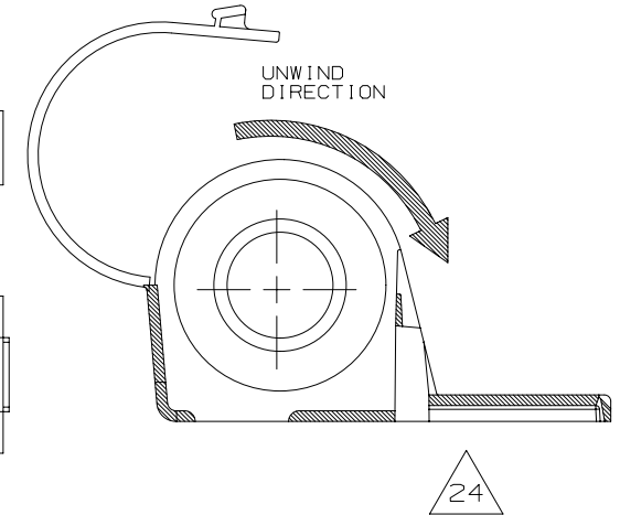
FIG. 2 FRONT VIEW
