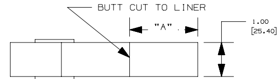
FIGURE 1. (TOP VIEW)
