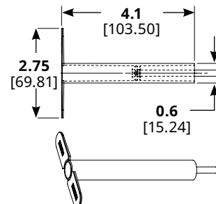
PZBR4 4 in. Bend Radius Post Kit
