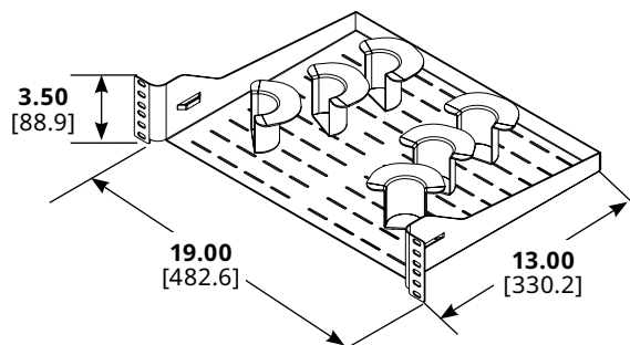
PZCHSM2 Horizontal Slack Manager, 2 RU includes (2) PZBR4 Kits
