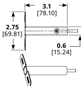
PZBR3 3 in. Bend Radius Post Kit
