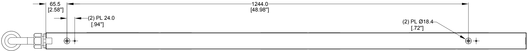
REAR VIEW
