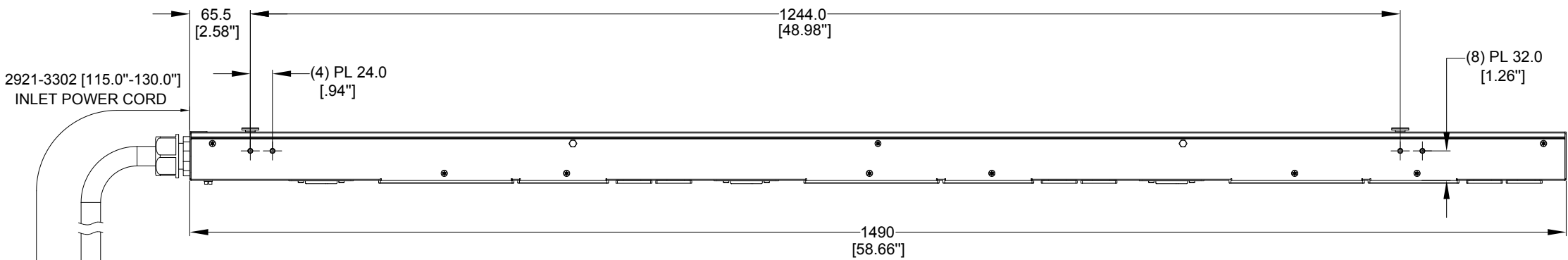
TOP VIEW
