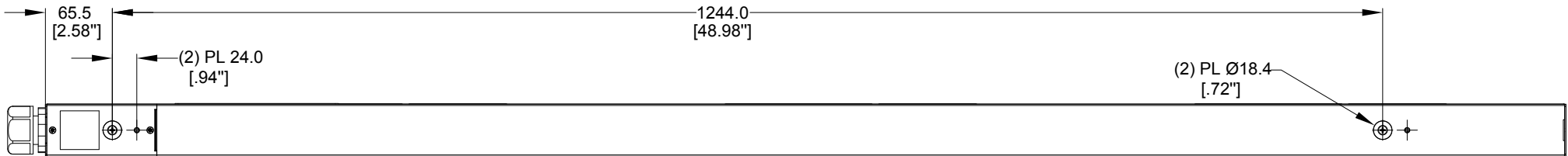
REAR VIEW
