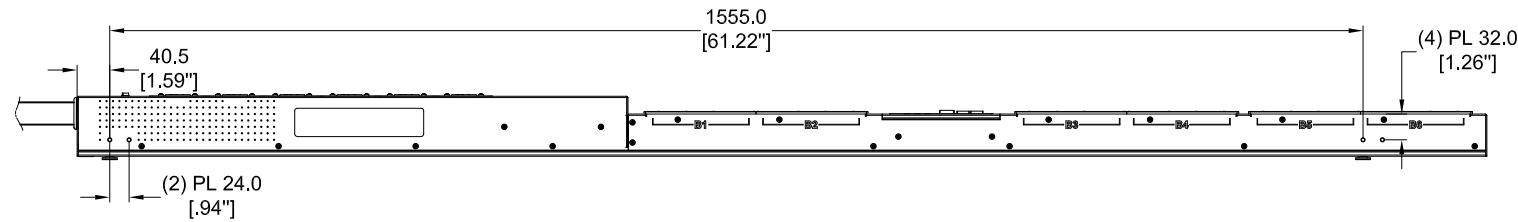
LEFT VIEW
