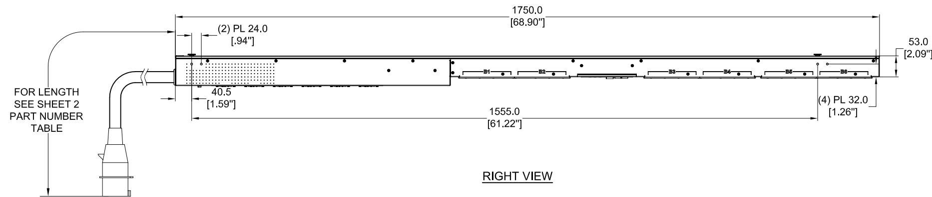
REAR VIEW
