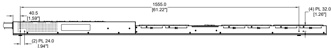
LEFT VIEW
