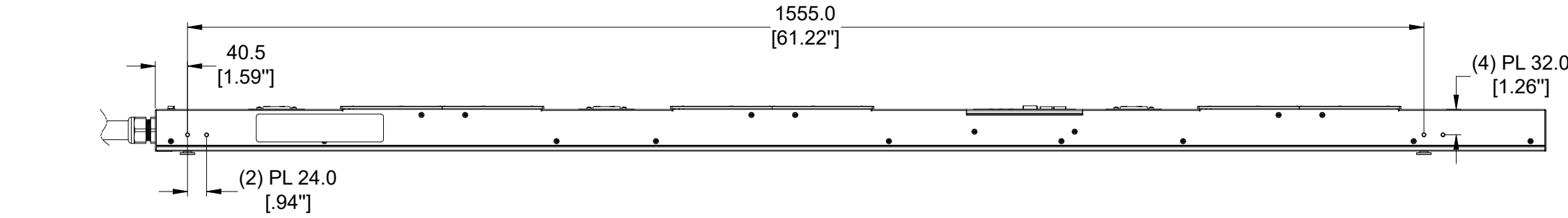
LEFT VIEW
