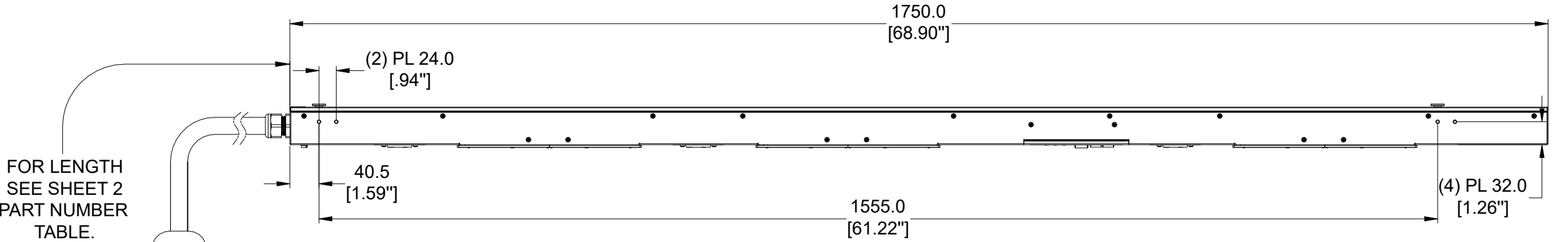
RIGHT VIEW
