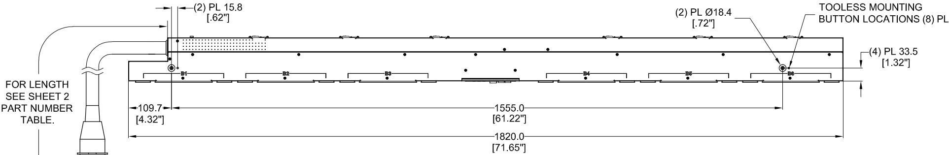
RIGHT VIEW
