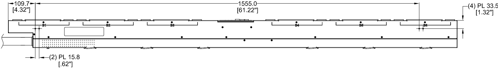
LEFT VIEW
