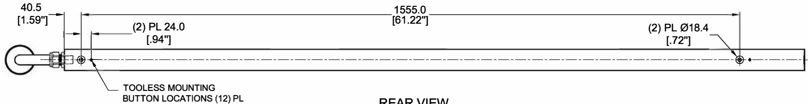
REAR VIEW
