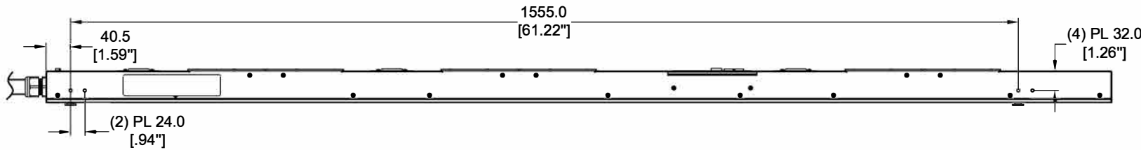
LEFT VIEW
