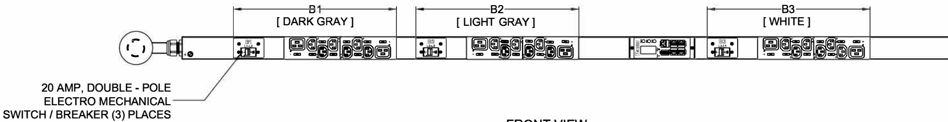
FRONT VIEW
