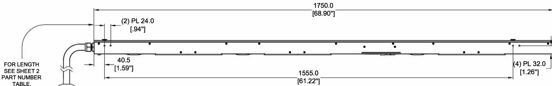
RIGHT VIEW
