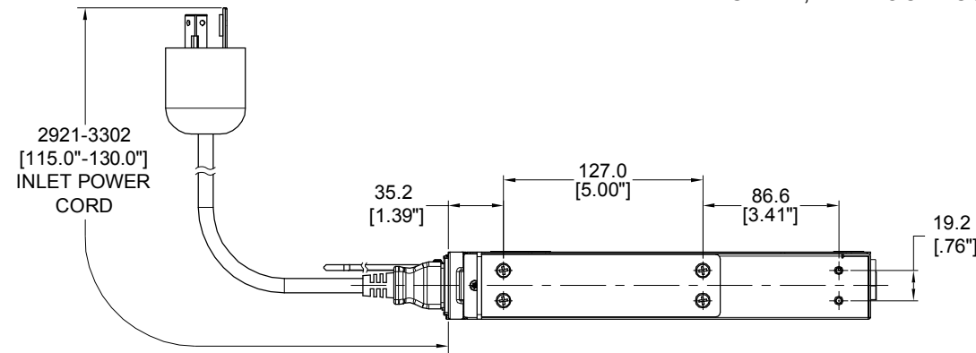
SIDE VIEW
