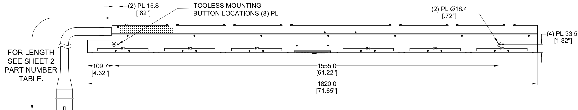
RIGHT VIEW
