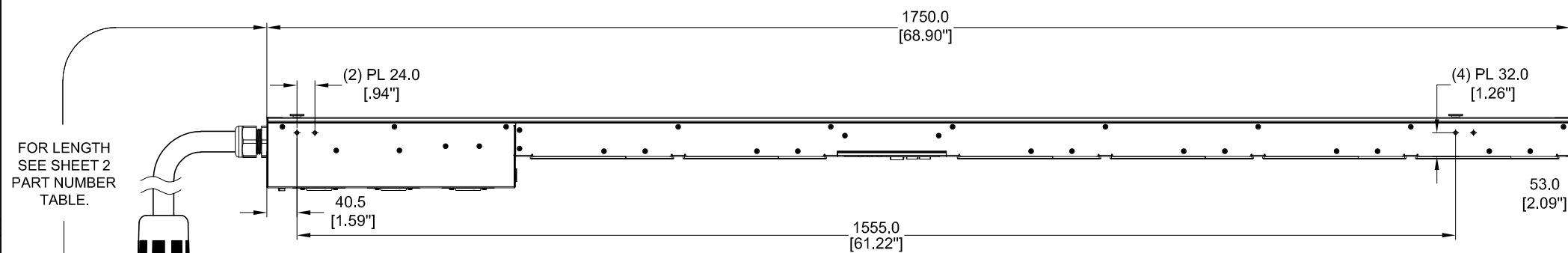
RIGHT VIEW
