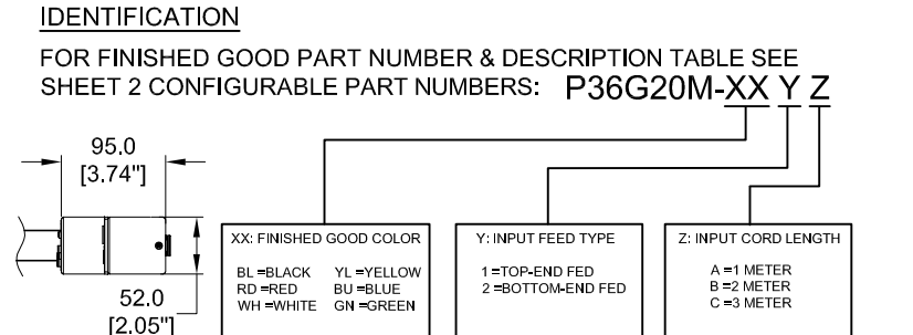
BOTTOM VIEW
