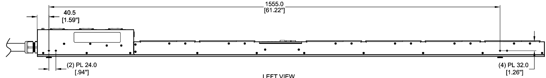
LEFT VIEW
