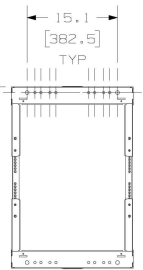
TOP VIEW 30" DEPTH
