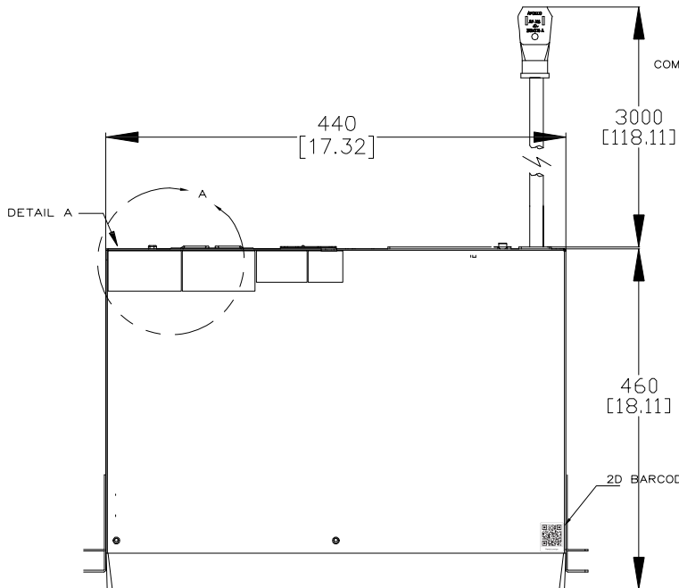
VIEW ROTATED 180
