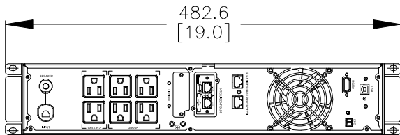
VIEW ROTATED 180
