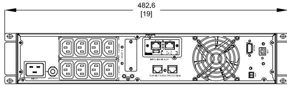
VIEW ROTATED 180°
