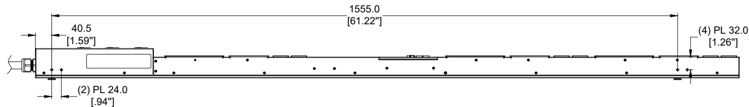
LEFT VIEW
