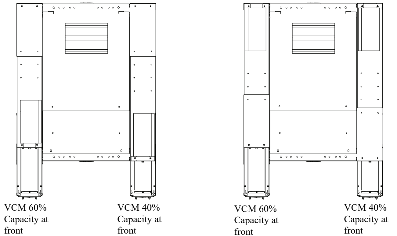
VCM Top Caps with Brush entry at the front of the rack
