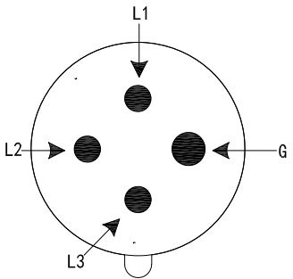
INPUT PLUG FRONT VIEW
