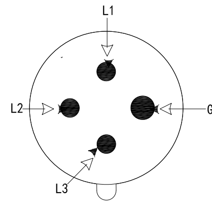
INPUT PLUG FRONT VIEW
