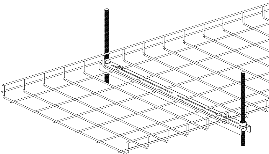
2' X 30' WIRE BASKET WITH TRAPEZE BRACKET SHOWN
