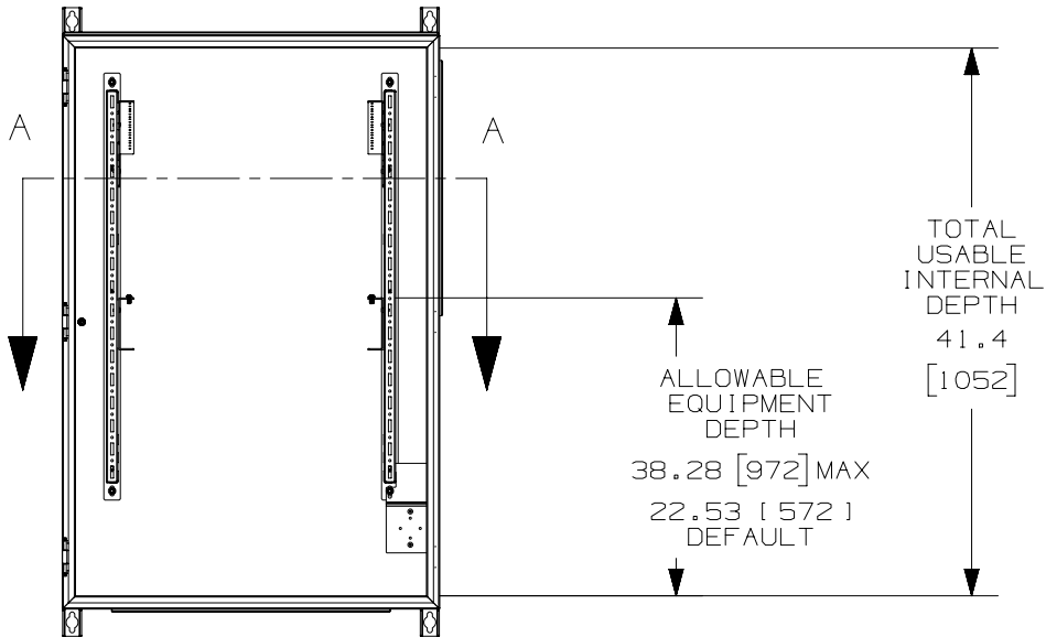
FRONT VIEW DOOR REMOVED
