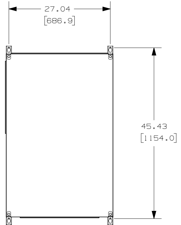
BACK VIEW
