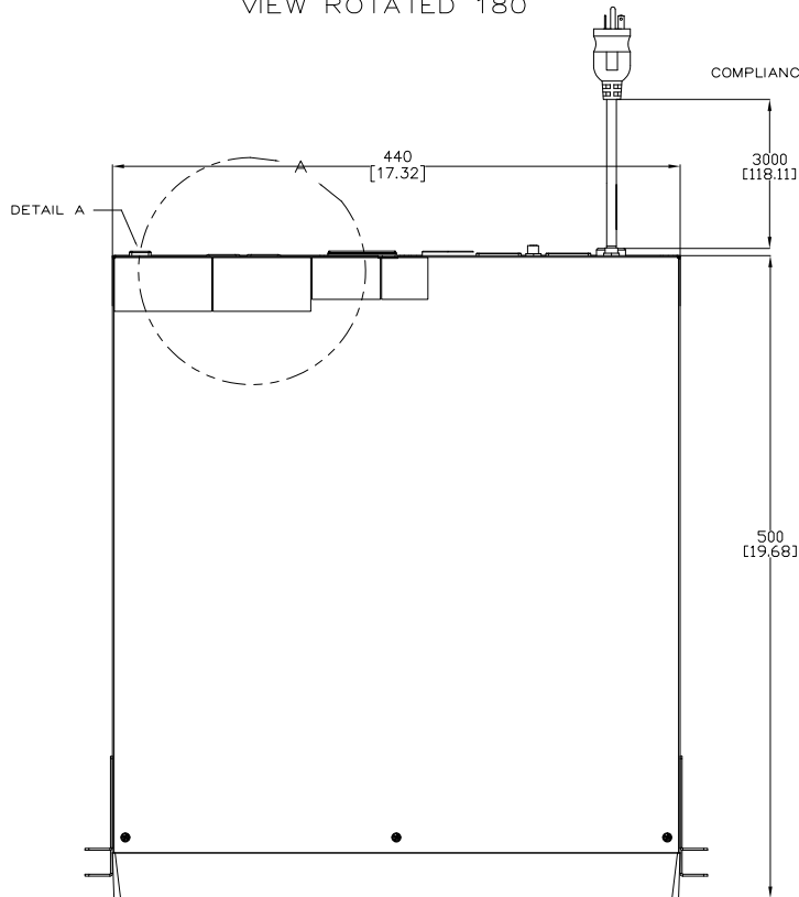
VIEW ROTATED 180°
