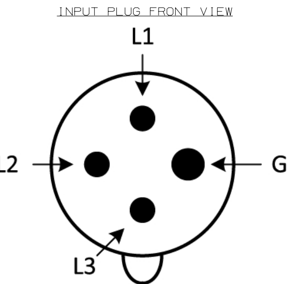
INPUT PLUG FRONT VIEW
