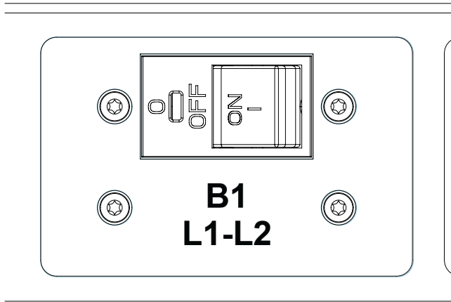
DETAIL A SCALE 1:1 CIRCUIT BREAKER ORIENTATION TYP 6X
