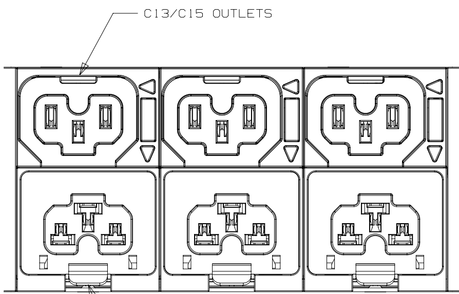
DETAIL B SCALE 1:1 C13/C15/C19/C21 OUTLETS
