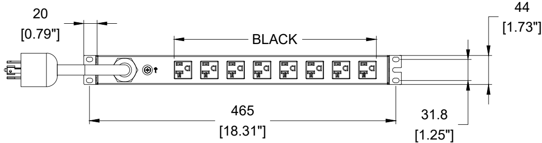
REAR VIEW
