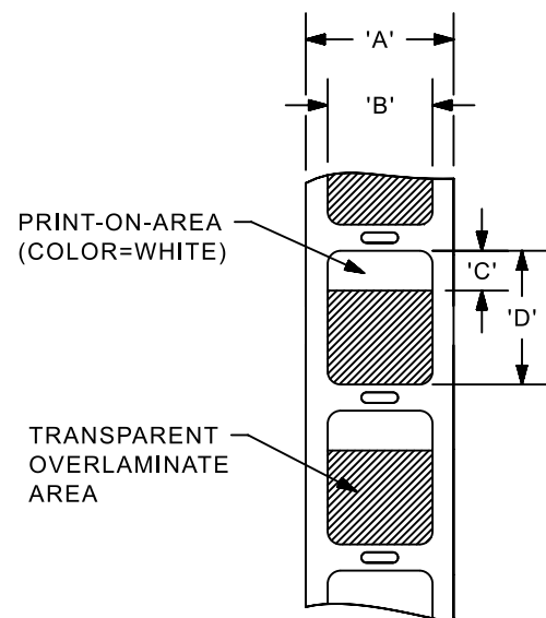
CASSETTE TYPE 1
