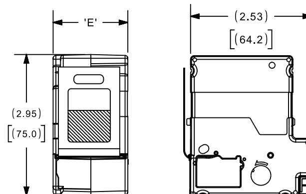
CASSETTE TYPE 1
