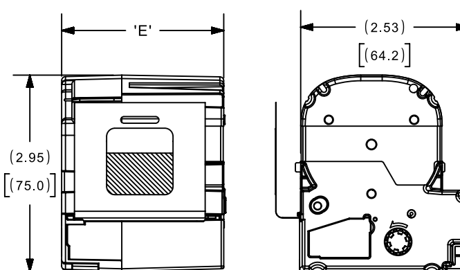
CASSETTE TYPE 2
