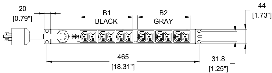
REAR VIEW
