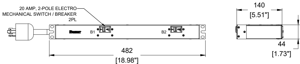
FRONT VIEW
