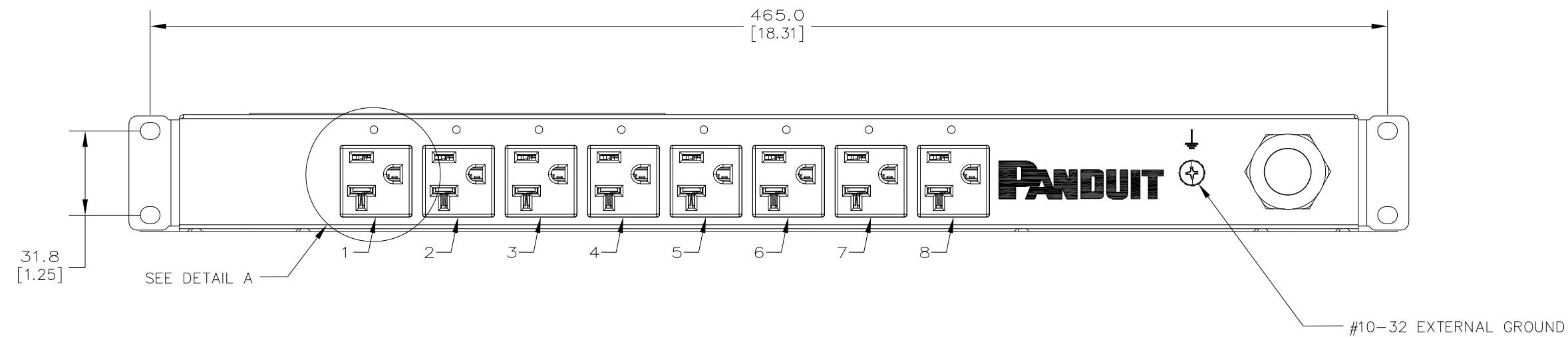
REAR VIEW
