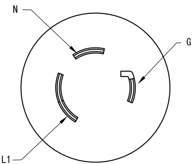
INPUT PLUG FRONT VIEW
