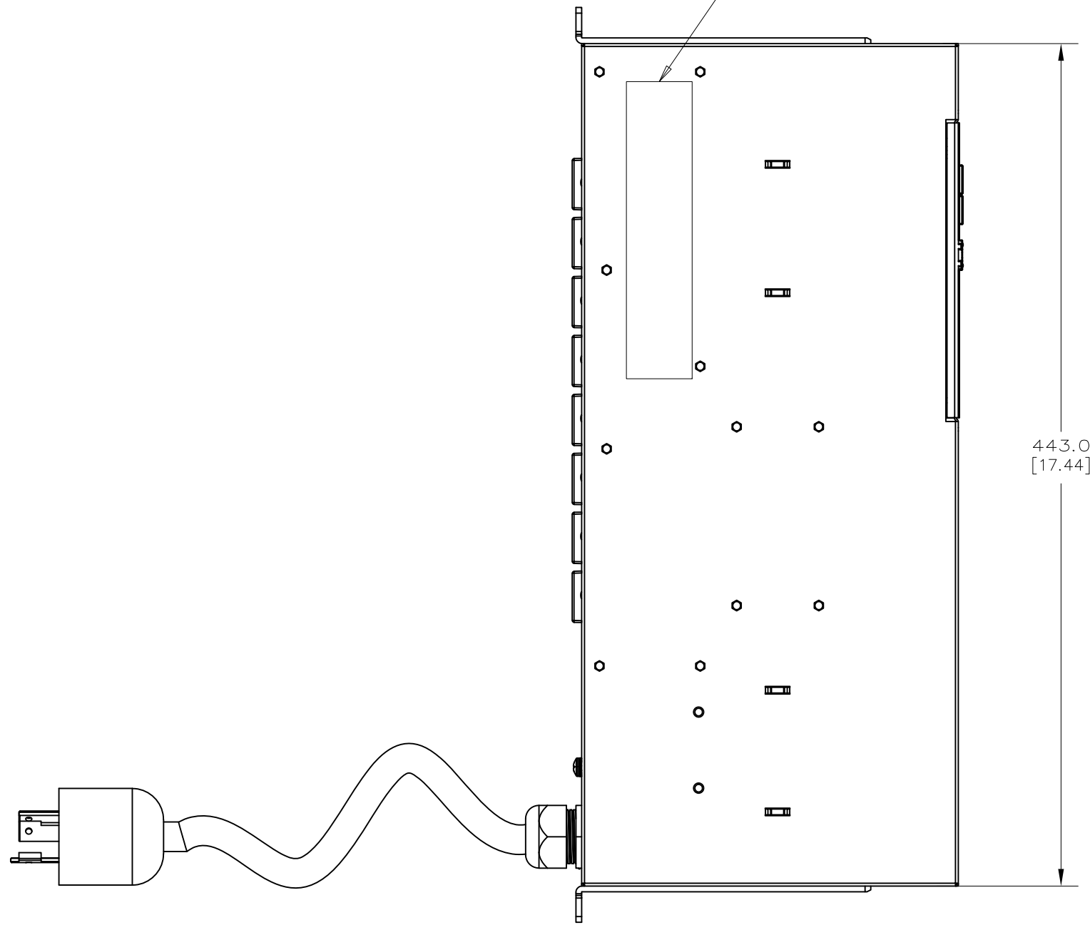
TOP VIEW
