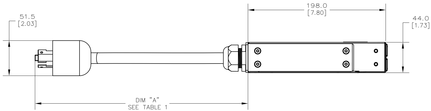
SIDE VIEW
