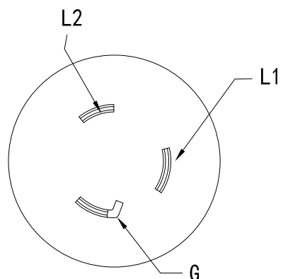
INPUT PLUG FRONT VIEW
