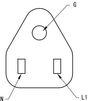
INPUT PLUG FRONT VIEW
