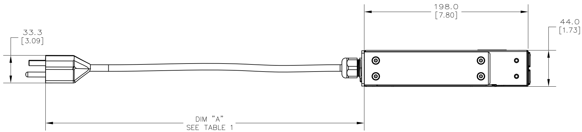
SIDE VIEW
