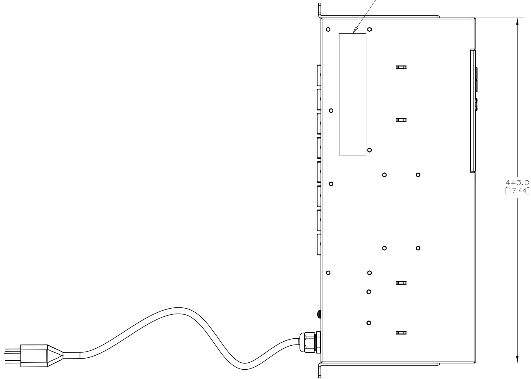
TOP VIEW
