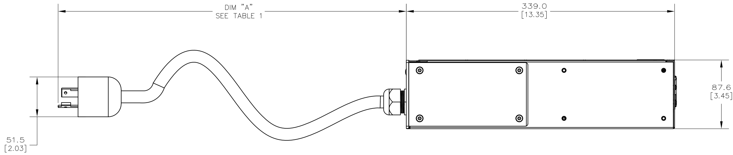
SIDE VIEW
