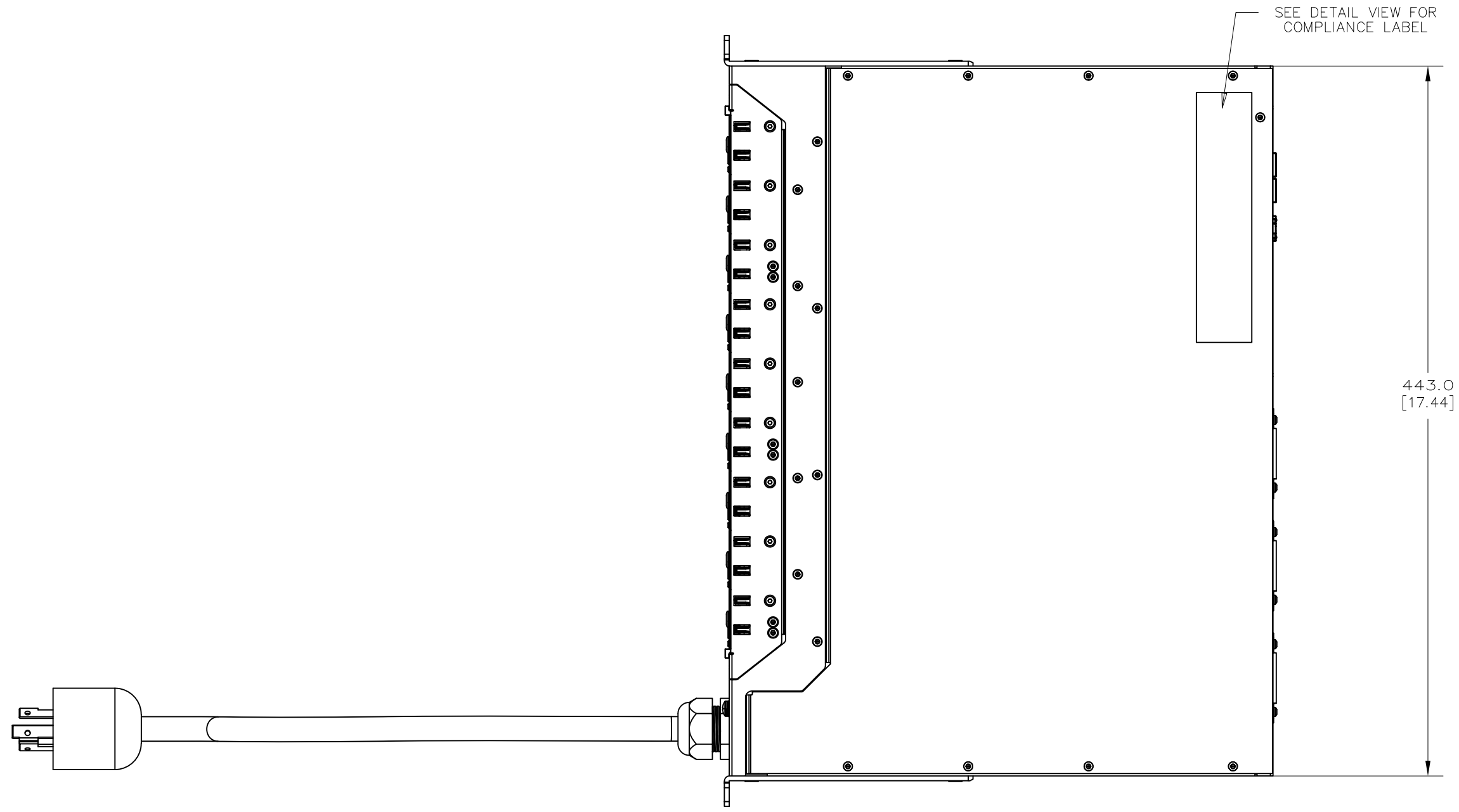
TOP VIEW
