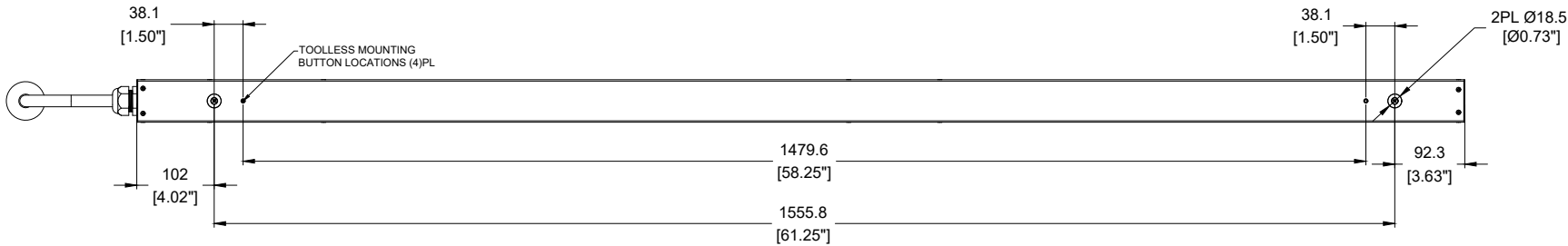
LEFT VIEW
