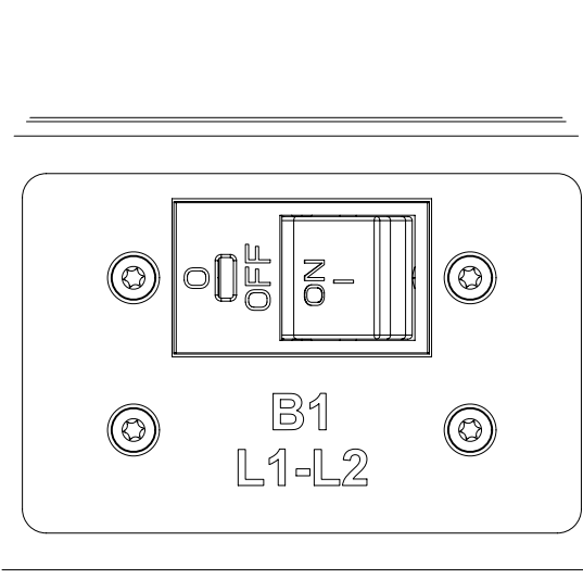
DETAIL A SCALE 1:1 CIRCUIT BREAKER ORIENTATION TYP 3X
