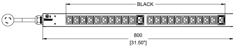
RIGHT VIEW
