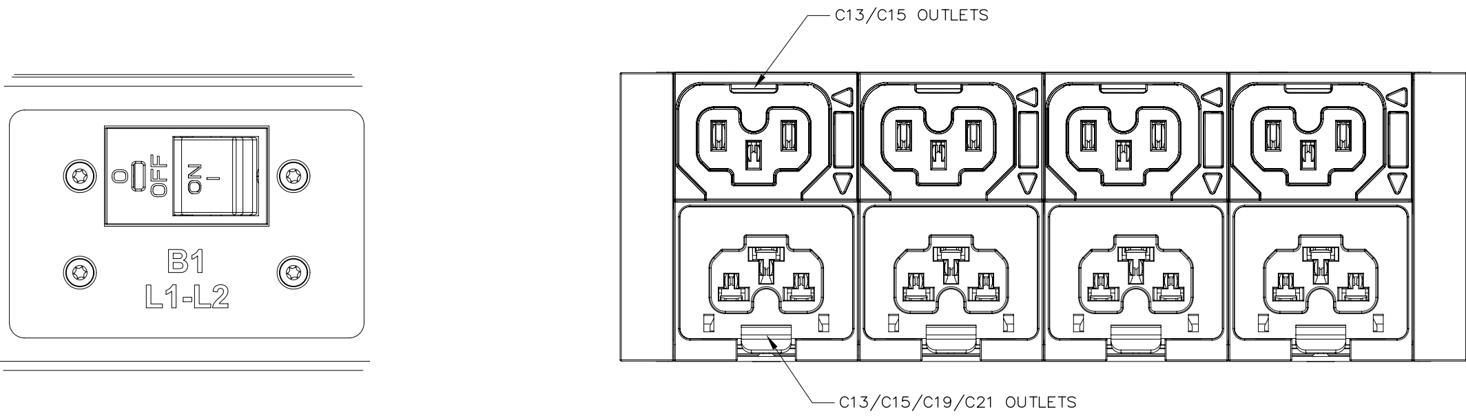
DETAIL A SCALE 1:1 CIRCUIT BREAKER ORIENTATION TYP 2X
