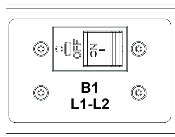
DETAIL A SCALE 1:1 CIRCUIT BREAKER ORIENTATION TYP 6X
