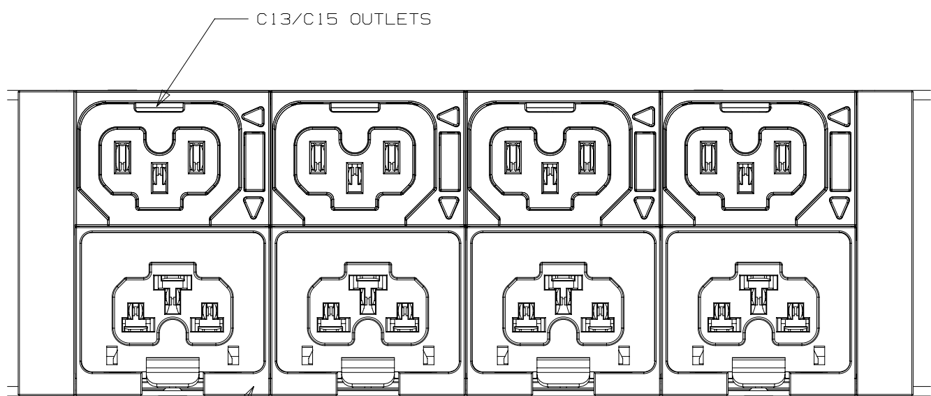
DETAIL B SCALE 1:1
