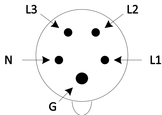
INPUT PLUG FRONT VIEW
