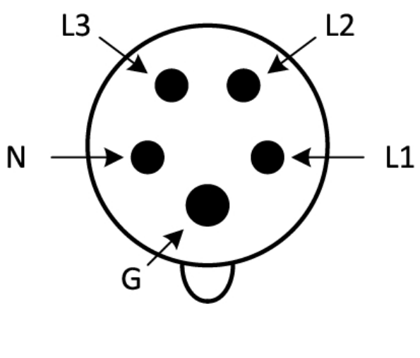
INPUT PLUG FRONT VIEW
