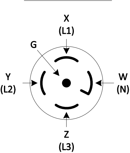
INPUT PLUG FRONT VIEW
