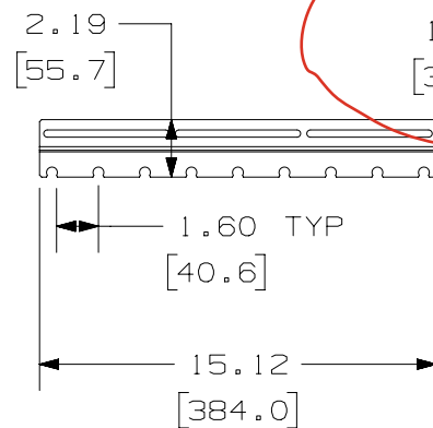
CABINET BRACKET
