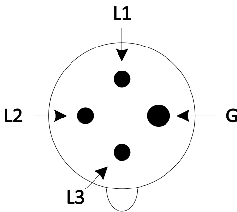
INPUT PLUG FRONT VIEW
