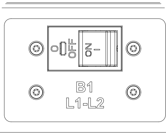
DETAIL A SCALE 1:1 CIRCUIT BREAKER ORIENTATION TYP 6X
