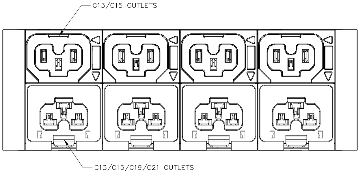
DETAIL B SCALE 1:1
