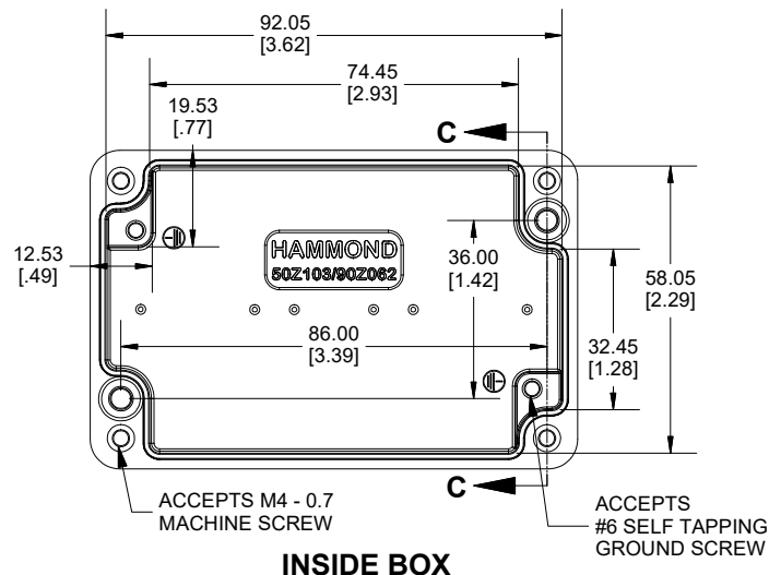
INSIDE BOX
