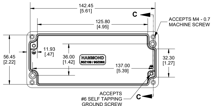
INSIDE BOX
