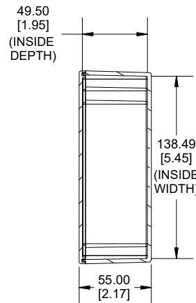
SECTION A-A END VIEW
