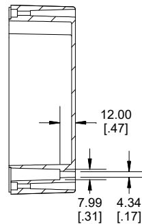
SECTION C-C MOUNTING HOLE
