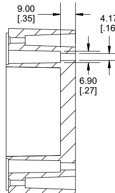
SECTION C-C MOUNTING HOLE
