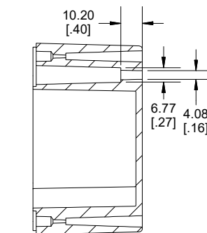
SECTION C-C MOUNTING HOLE
