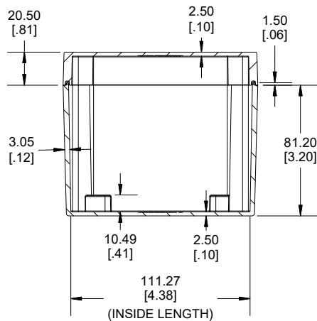
SECTION B-B SIDE VIEW
