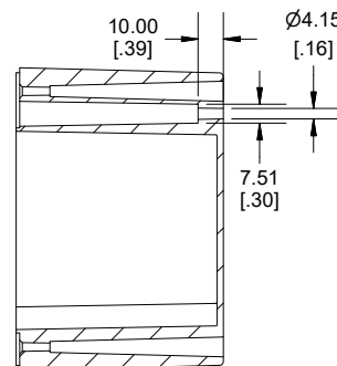
SECTION C-C MOUNTING HOLE
