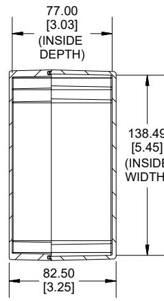
SECTION A-A END VIEW
